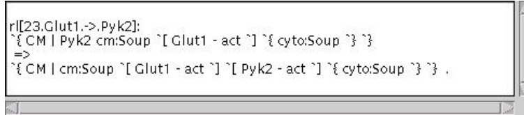
Fig. 3. The result of invoking the show rule action
